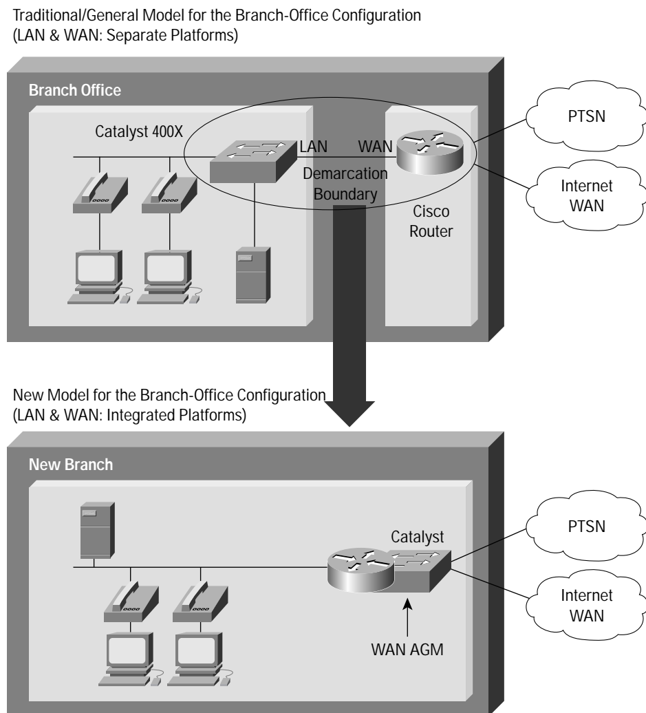
Figure 4 Cisco Catalyst 4000 Family Branch-Office Solution
